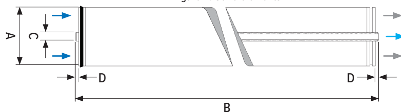
Figure 2: 8040 elements
