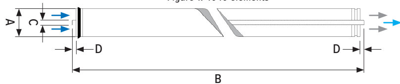
Figure 1: 4040 elements
